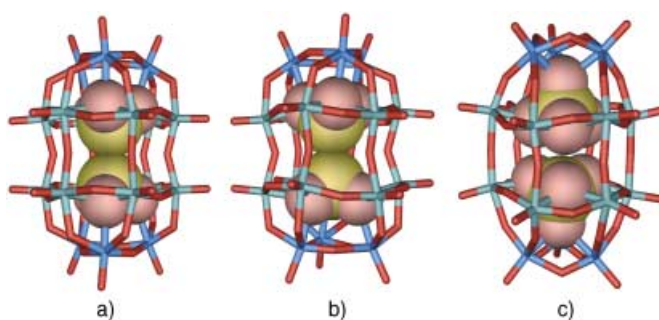
Figure 1. A representation of the structures of the sulfite-based Dawson clusters: a) \alpha-[Mo_2^V Mo_{16}^{VI} O_{54}(SO_3)_2]^{6-} ( 1a ), b) \beta-[Mo_{18}^{VI} O_{54}(SO_3)_2]^{4-} ( 3a ), and c) a comparison with the conventional \alpha -type sulfate-based Dawson anion [Mo_{18}O_{54}(SO_4)_2]^{4-} , [6] whereby the central anion templates are shown in a space-filling mode (S: yellow, O: red, capping Mo: blue, “belt” Mo: green).
